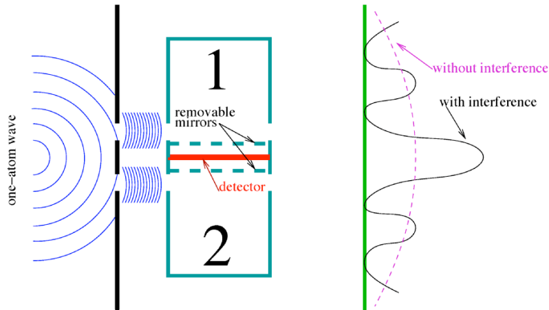
Fig. 1: The Quantum Eraser arrangement.
